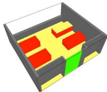
Fig. 3. An impression of the FDS simulation model (the four red areas are beds) and different simulation scenario's
