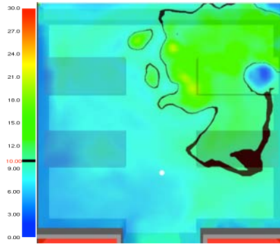
Fig. 5. Soot visibility of model #1 with a RHR of 100 \text{ kW/m}^2 and a time constant of 300 seconds, at 155 seconds. The black line indicates the transition zone from a visibility of 10 metres or higher to a lower value
