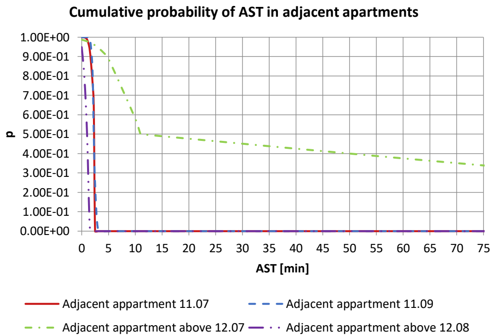
Figure 5-8. Cumulative probability of ASET in adjacent compartments.
