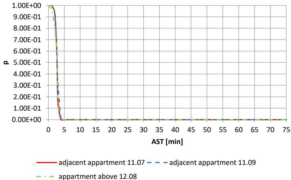
Figure 5-7. Cumulative probability of AST in adjacent compartments.
