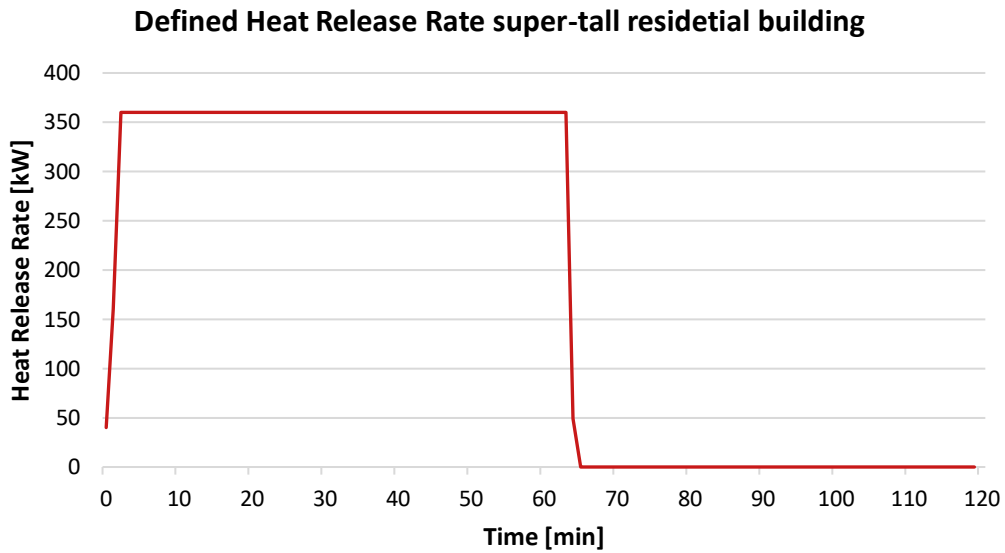
Figure 9-5. Defined Heat Release Rate in a sprinklered compartment of the super-tall residential building.
