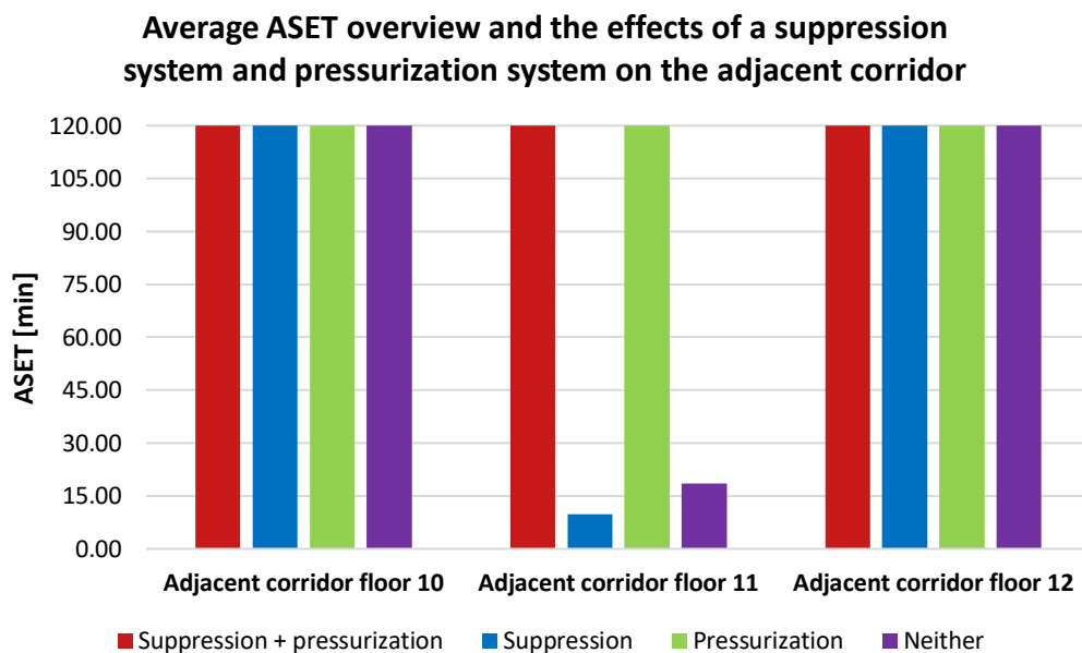
Figure 5-14. Average ASET overview and the effect of a suppression system and pressurization system on the adjacent corridor.
