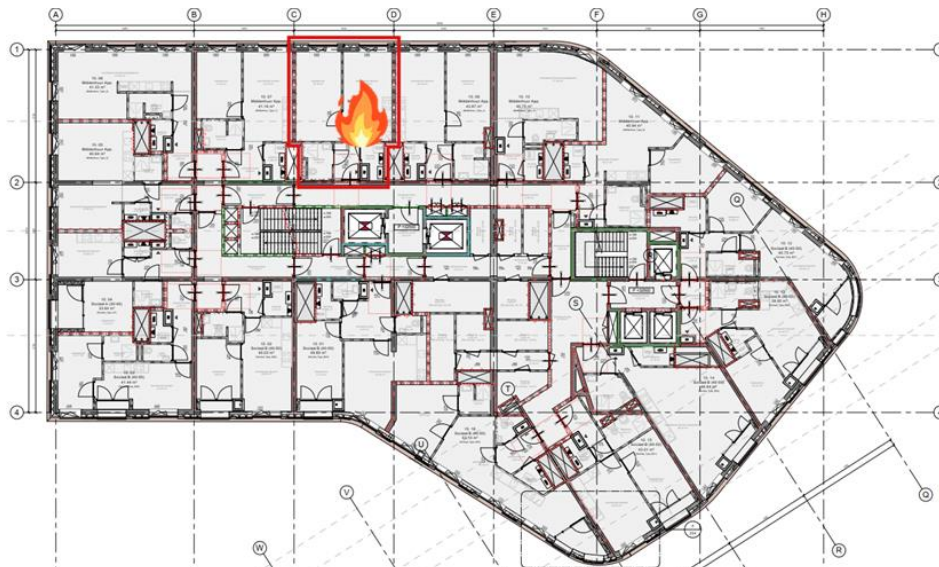
Figure 9-1. Geometry of the 10 th -13 th floor, and the compartments used in the Ozone calculations.
