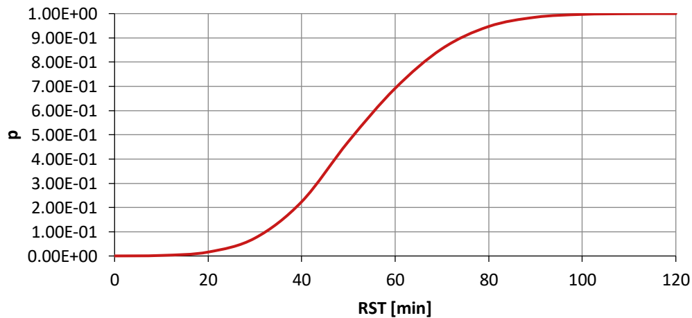
Figure 5-6. Cumulative probability of thermal action on compartment separation constructions.
