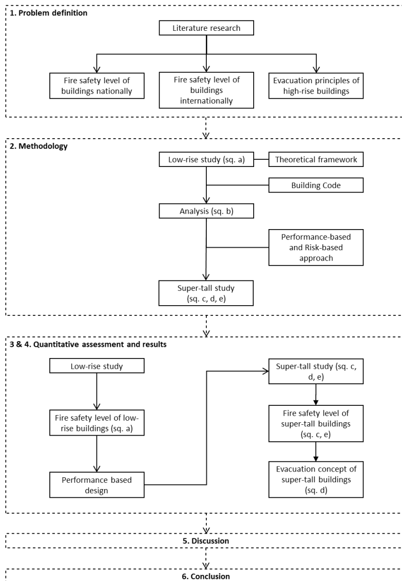
Figure 2-1. Research methodology.
