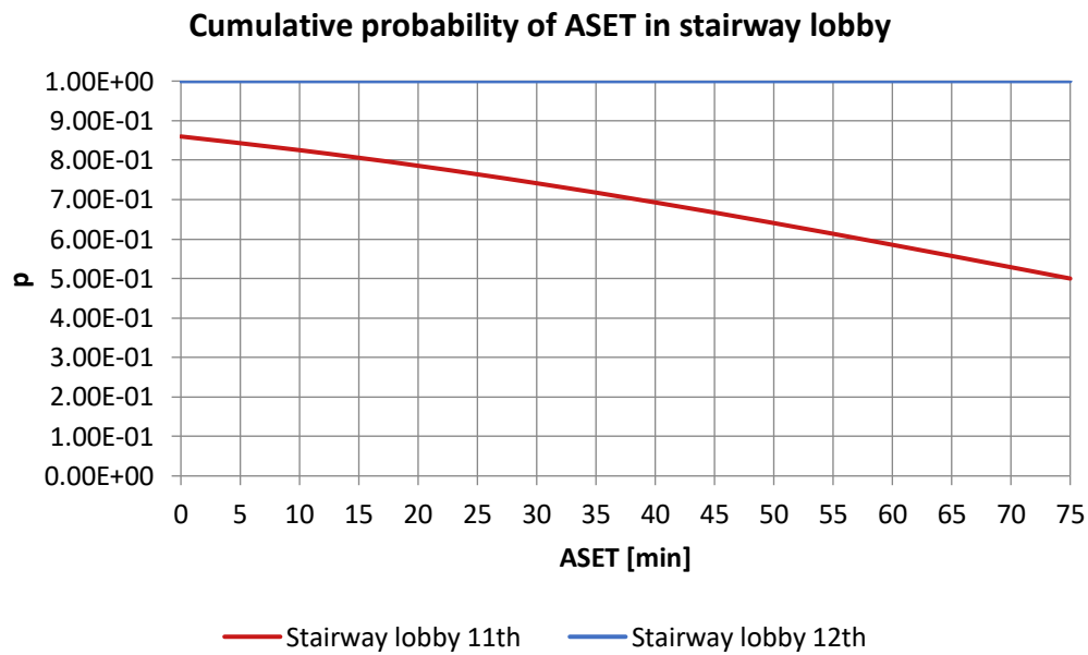
Figure 5-12. Cumulative probability of ASET in stairway lobby.
