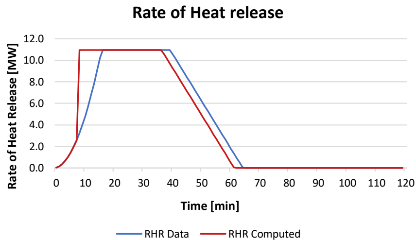
Figure 2-4. Rate of Heat Release (RHR) of natural fire according to Annex E of NEN-EN 1991-1-2/NB, used in the Ozone model.
