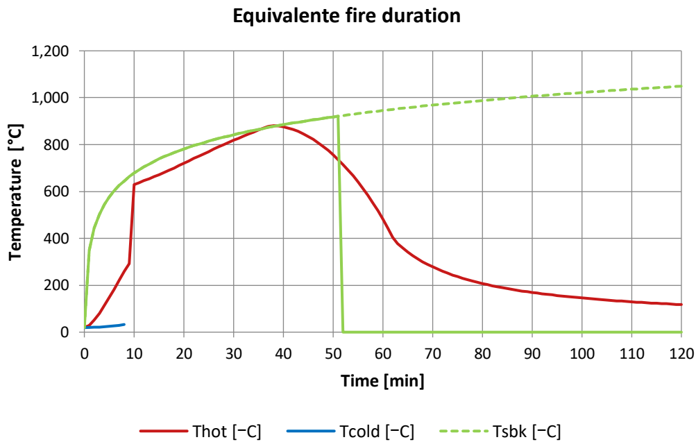
Figure 5-5. Equivalent fire duration for the low-rise residential reference building and the super-tall residential building.
