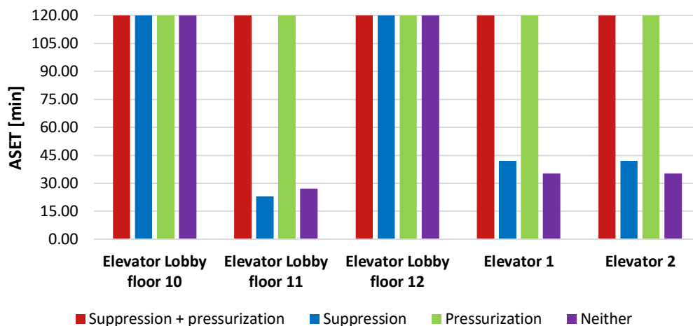
Figure 5-16. Average ASET overview and the effect of a suppression system and pressurization system on the elevator lobbies and elevators.
