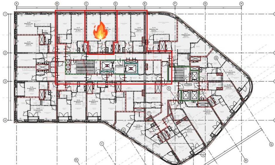
Figure 9-2. Geometry of the 10 th – 13 th floor, and the lay-out for the CFAST calculations.
