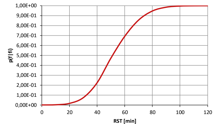
Cumulative probability of thermal action on compartment separation constructions
