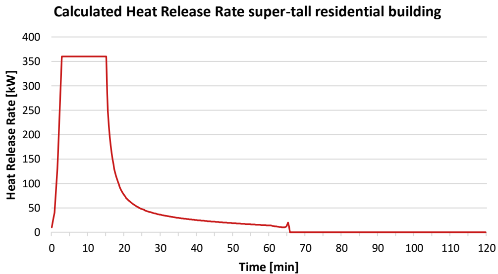
Figure 9-6. Calculated Heat Release Rate in a sprinklered compartment of the super-tall residential building.
