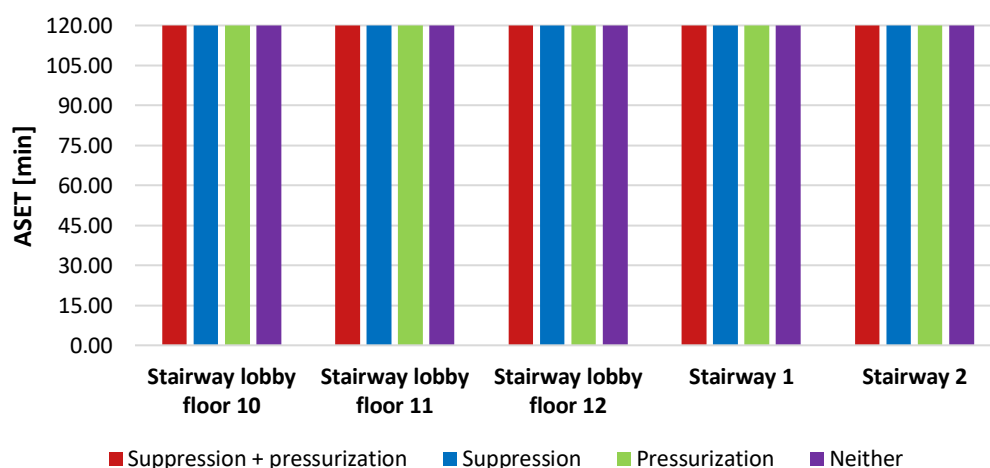
Figure 5-15. ASET overview and the effect of a suppression system and pressurization system on the stairway lobby and stairway.
