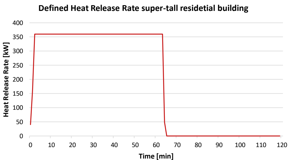
Figure 5-3. Defined Heat Release Rate in a sprinklered compartment of the super-tall residential building.
