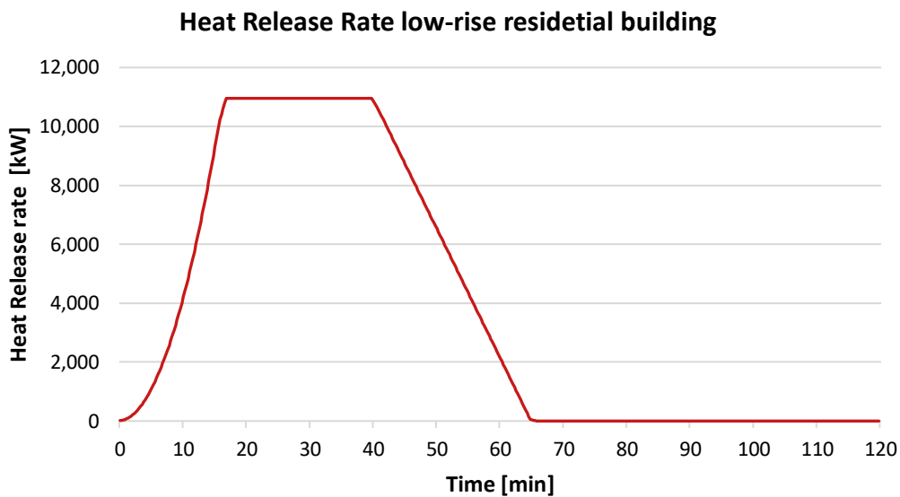
Figure 5-2. Heat release rate of a fire in a compartment of the low-rise residential reference building.
