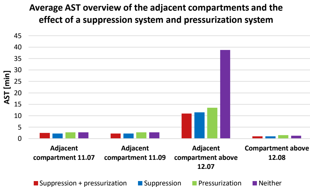
Figure 5-9. Average AST overview and the effect of a suppression system and a pressurization system on the adjacent compartment.
