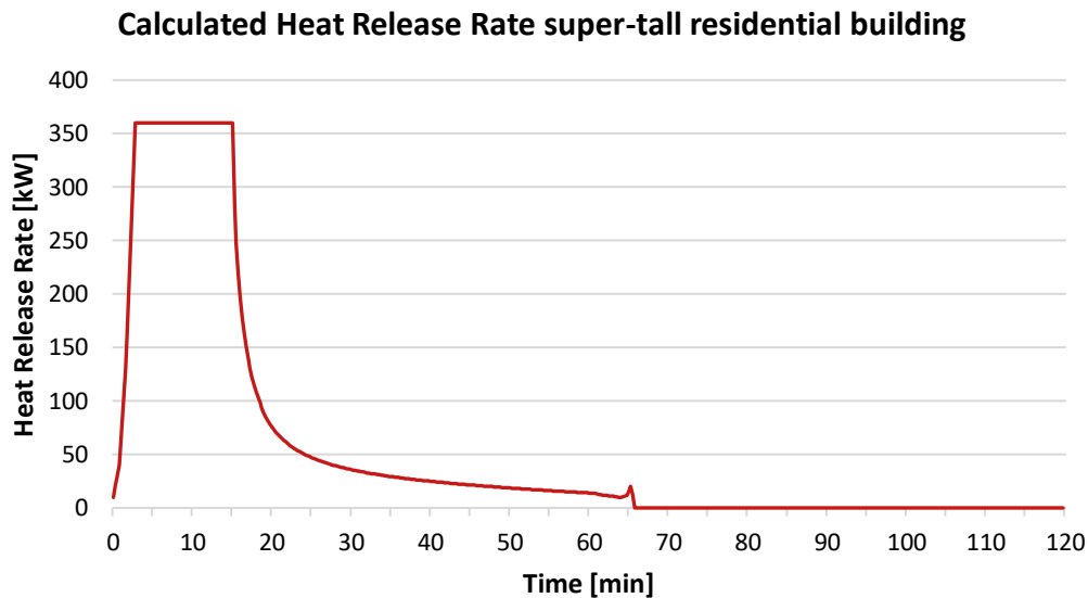
Figure 5-4. Calculated Heat Release Rate in a sprinklered compartment of the super-tall residential building.
