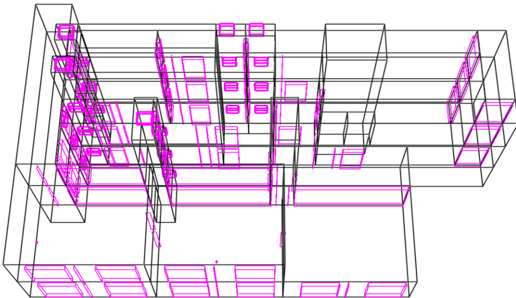
Figure 9-4. Geometry (wire model in 3D) of the super-tall study simulations in Smokeview.
